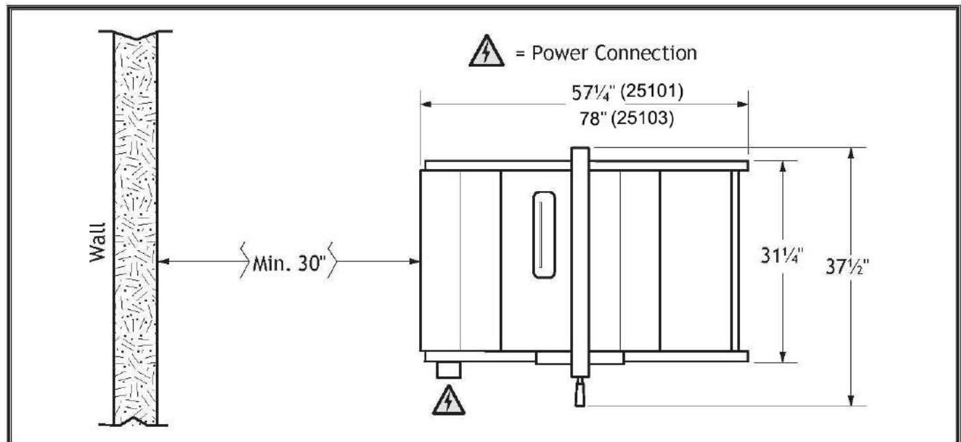
Figure 11. Working clearances.
