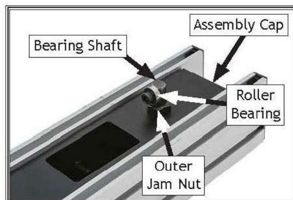
Figure 116. Rear adjustment area for leveling fence.
