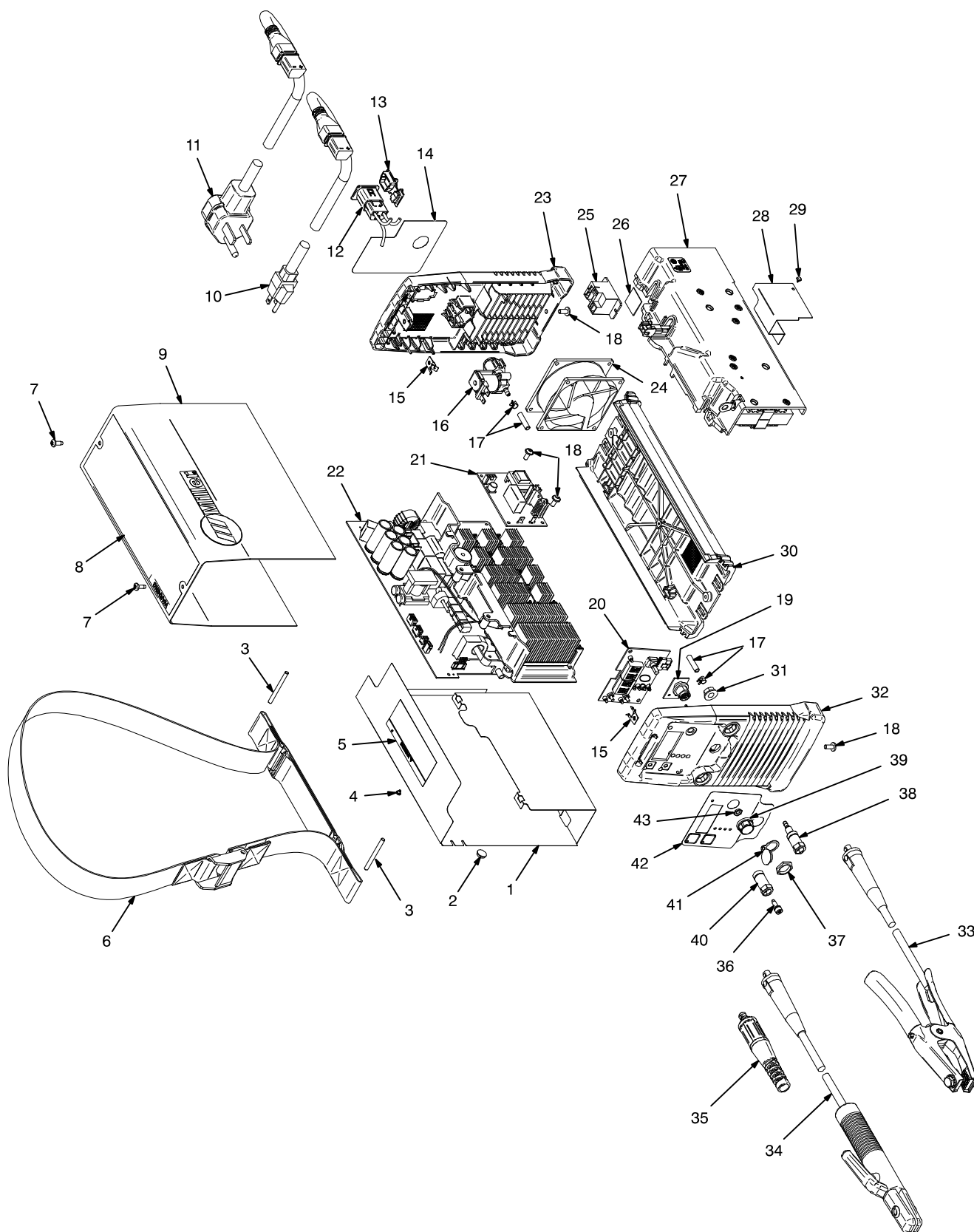
Figure 3-1. Main Assembly
