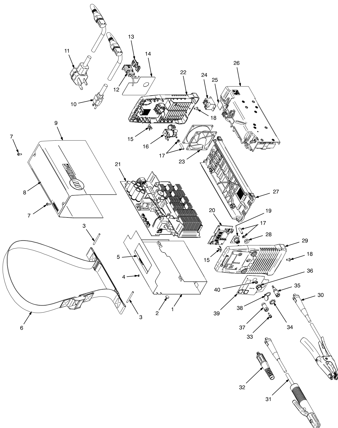
Figure 2-1. Main Assembly
