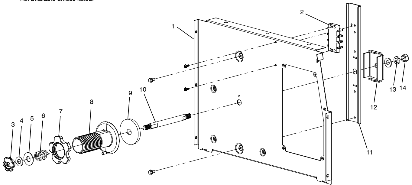
Figure 1-2. Center Baffle Assembly (Figure 1-1 Item 2)
