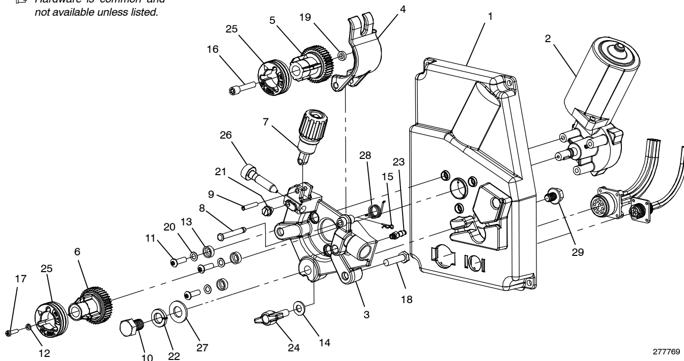
Figure 1-5. Wire Feed Drive Assembly (Figure 1-1 Item 5)
