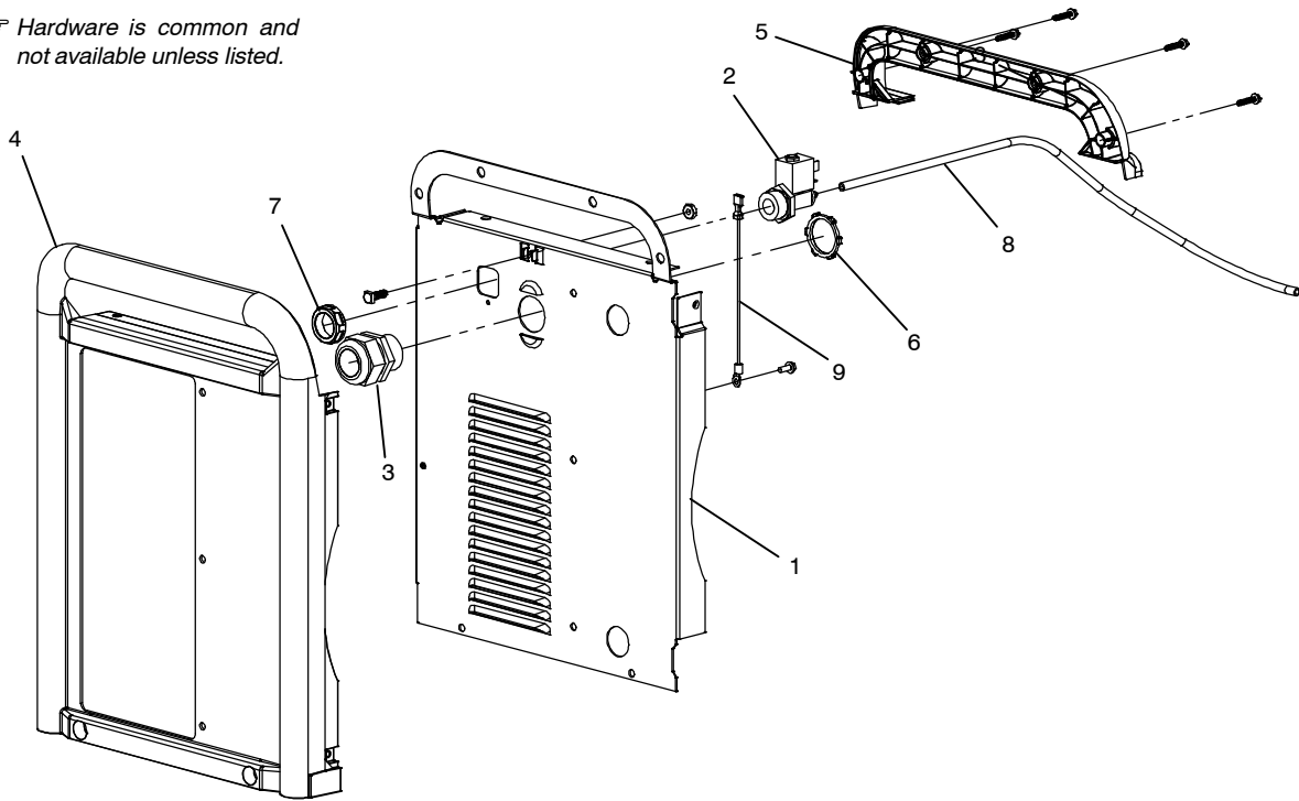
Figure 1-4. Rear Panel Assembly (Figure 1-1 Item 4)
