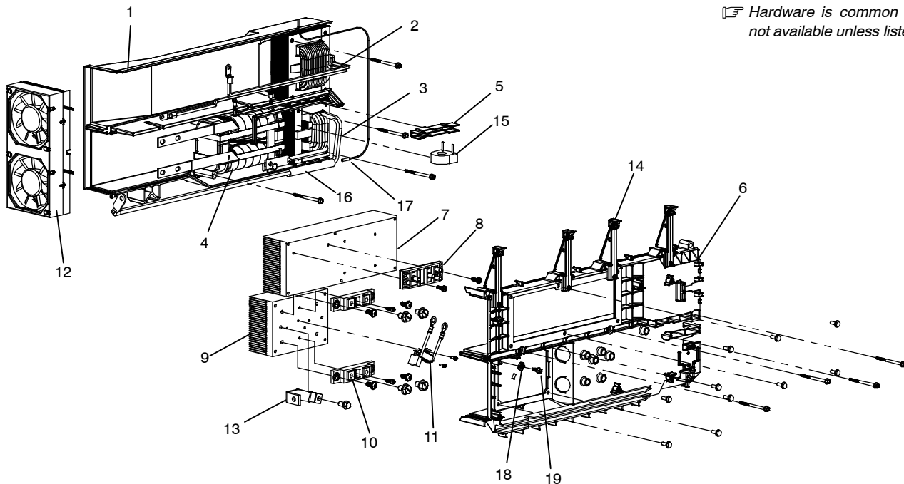
Figure 1-6. Windtunnel Assembly (Figure 1-1 Item 6)
