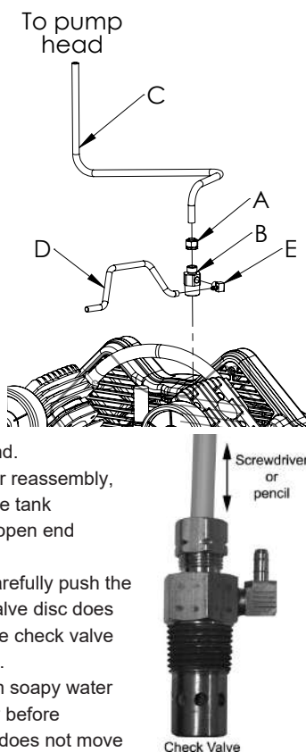
Check Valve
