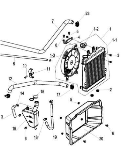
9 冷却水箱 Cooling water tank
