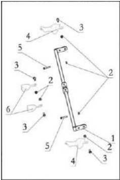
14 SAFETY BELT ASSY 安全带总成
