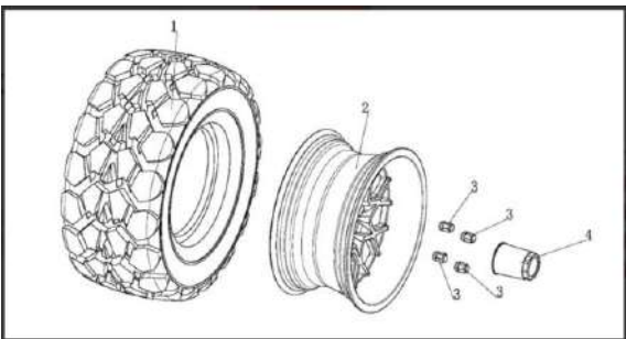
17 WHEEL SYSTEM 轮胎
