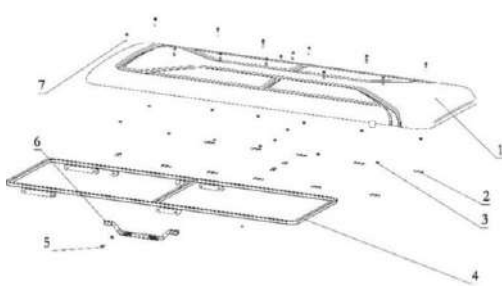
13 ROOF ASSY 顶棚装配
