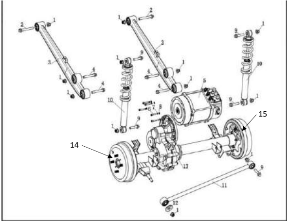
11 REAR SUSPENSION 后悬挂
