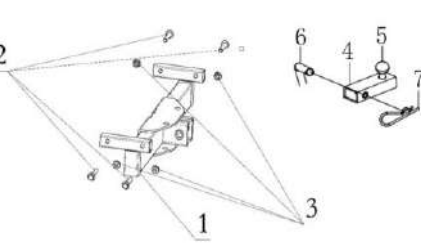
16 TRAILER HOOK ASSY 拖挂装配
